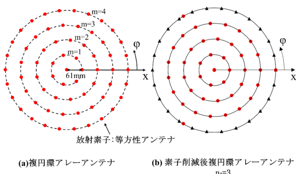
Figure 1: Antenna Configuration
