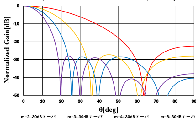
Figure 2: Radiation Pattern with Quadratic Distribution
